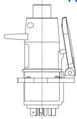
7'Lİ N TİPİ ALÜMİNYUM TIR RÖMORK PRİZİ (TERMİNALLI VE SOKETLİ) / 7 PIN ALUMINIUM TIR TRAILER SOCKET (N TYPE)
