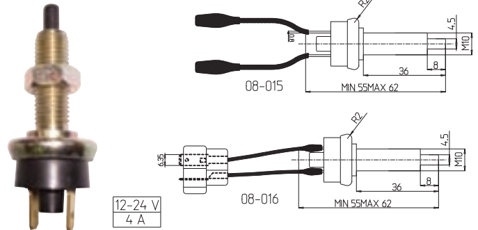
MITSUBISHI CANTER 459-659 - HYUNDAI H-100 FREN OTOMATİĞİ / STOPLIGHT SWITCH ISUZU NPR / NKR / TFR FREN OTOMATİĞİ STOPLIGHT SWITCH
