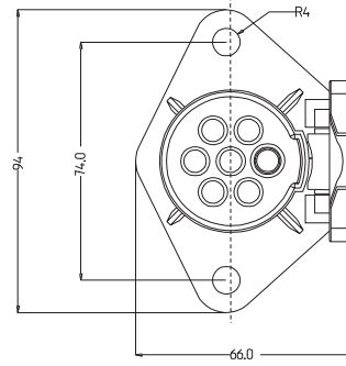
7'Lİ N TİPİ PLASTİK TIR RÖMORK FİŞİ (TERMİNALLİ VE SOKETLİ) / 7 PIN PLASTIC TIR TRAILER PLUG (N TYPE)
