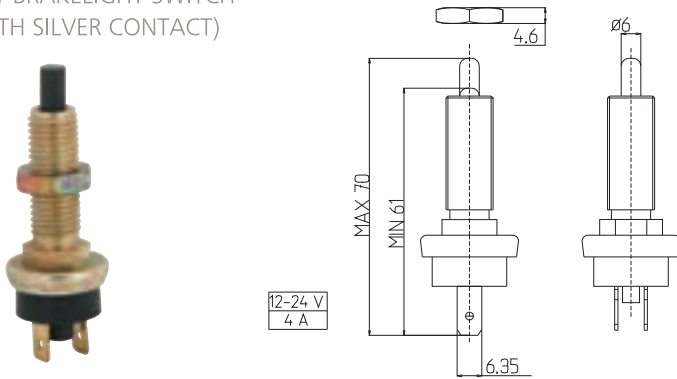
ESKİ MODEL CLİO / KANGOO 2 FİŞLİ ORJİNAL YENİ MODEL CLİO / KANGOO 4 FİŞLİ ORJİNAL OLD/NEW MODEL CLIO/KANGOO 2/4 SOCKET
