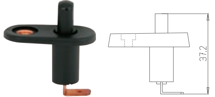
BUTON KAPI VE ALARM İÇİN (PLASTİK KISA) PUSH BUTTON FOR DOOR AND ALARM (PLASTIC SHORT)
