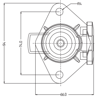
7'Lİ N TİPİ ALÜMİNYUM TIR RÖMORK PRİZİ (TERMİNALLI VE SOKETLİ) / 7 PIN ALUMINIUM TIR TRAILER SOCKET (N TYPE)
