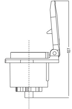
7'Li N TİPİ ALÜMİNYUM TIR RÖMORK FİŞİ (VİDALI) / 7 PIN ALUMINIUM TIR TRAILER SOCKET (N TYPE AND SCREW TERMINAL)
