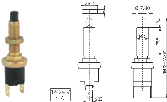
FIAT 131 FREN OTOMATİĞİ (PLASTİK) FIAT 131 STOPLIGHT SWITCH (PLASTIC)
