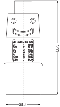
7'Li N TİPİ ALÜMİNYUM TIR RÖMORK PRİZİ (VİDALI) / 7 PIN ALUMINIUM TIR TRAILER (N TYPE AND SCREW TERMINAL)
