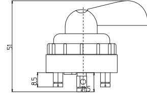
IŞIKLI SAĞ-SOL SİNYAL ANAHTARI / ON/OFF/ON THREE POSITION ROTARY SWITCH WITH GREEN ILLUMINATED LED
