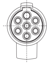
7'Li N TİPİ ALÜMİNYUM TIR RÖMORK PRİZİ (VİDALI) / 7 PIN ALUMINIUM TIR TRAILER (N TYPE AND SCREW TERMINAL)
