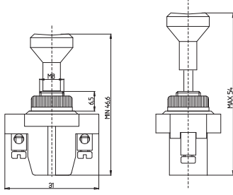
TEKLİ ÇEKME LAMBA ANAHTARI KISA PASO SHORT PUSH-PULL SWITCH
