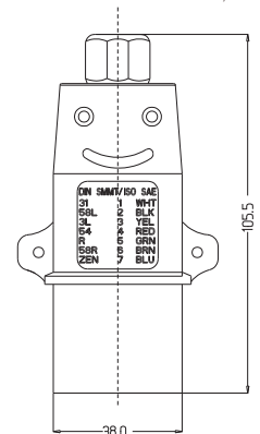
7'Li N TİPİ ALÜMİNYUM TIR RÖMORK FİŞİ (VİDALI) / 7 PIN ALUMINIUM TIR TRAILER SOCKET (N TYPE AND SCREW TERMINAL)
