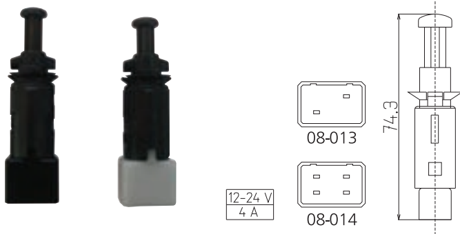
ESKİ MODEL CLİO / KANGOO 2 FİŞLİ ORJİNAL YENİ MODEL CLİO / KANGOO 4 FİŞLİ ORJİNAL OLD/NEW MODEL CLIO/KANGOO 2/4 SOCKET
