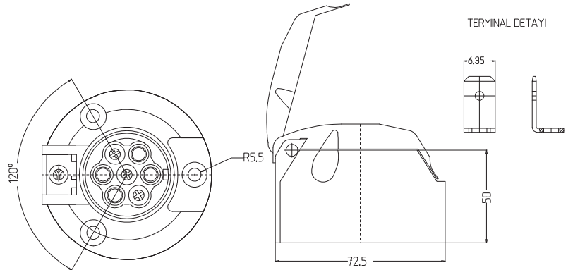
7'Lİ N TİPİ PLASTİK TRAKTÖR RÖMORK FİŞ VE PRİZ TAKIMI (FİŞ VİDALI, PRİZ TERMİNALLİ) 7 PIN TRAILER PLUG & SOCKET (N TYPE, COUPLE PLUG SCREW TYPE, SOCKET TERMINAL TYPE)
