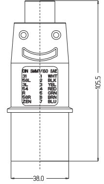
7'Li S TİPİ PLASTİK TIR RÖMORK FİŞİ (VİDALI) / 7 PIN PLASTIC TIR TRAILER SOCKET (S TYPE AND SCREW TERMINAL)
