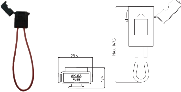
SİGORTA YUVASI KAPAKLI (ALTAN ÇIKIŞLI KABLOLU) FUSE HOLDER BLADE TYPE (WITH CABLE) 01-015
