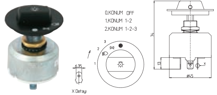
FORD KARGO FAR ANAH. (Y.M. ÇEVİRMELİ 32-30) 11-014 FORD CARGO HEADLIGHT ROTARY SWITCH (NEW MODEL)
