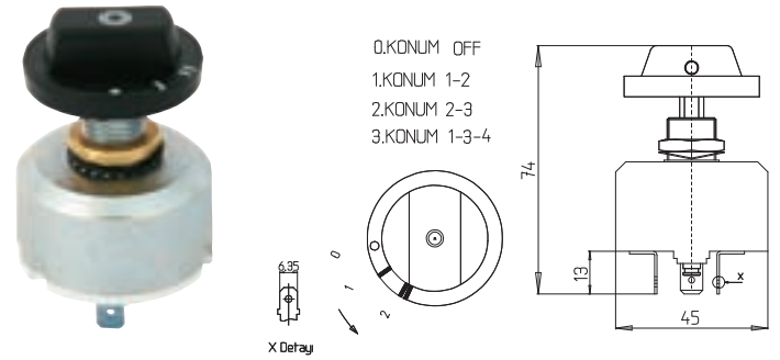
MAGIRUS KALORİFER ANAHTARI (Y.M. ÇEVİRMELİ) 11-018 MAGIRUS HEATING SYSTEM ROTARY SWITCH (NEW MODEL)
