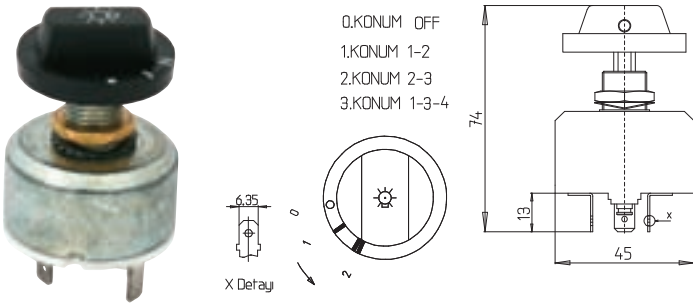
FORD KARGO FAR ANAH. (E.M. ÇEVİRMELİ 25-24) 11-013 FORD CARGO HEADLIGHT ROTARY SWITCH (OLD MODEL)
