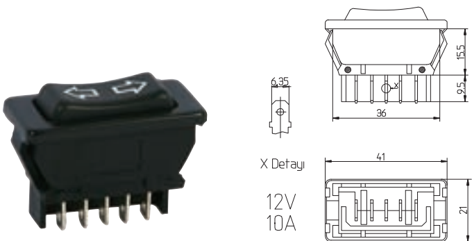
CAM VE ANTEN AÇMA-KAPAMA ANAHTARI 12 V. 20 A. 11-009 ELECTRIC WINDOW/AERIAL ROCKER SWITCH
