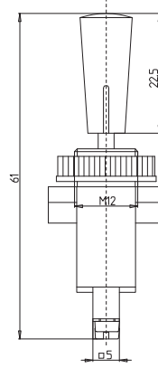
IŞIKLI SAĞ-SOL SİNYAL ANAHTARI / ON/OFF/ON THREE POSITION ROTARY SWITCH WITH GREEN ILLUMINATED LED
