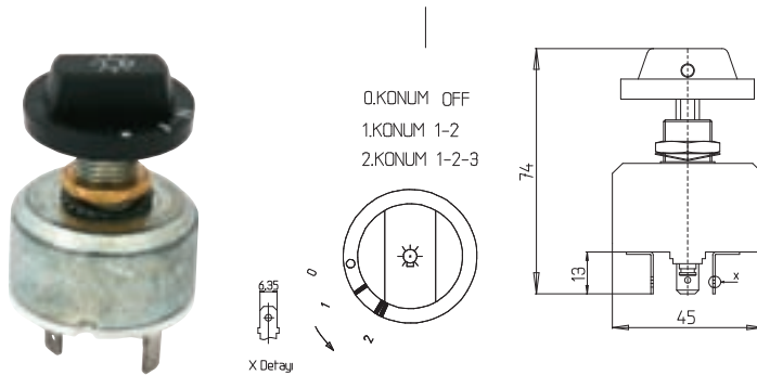
MAGIRUS FAR ANAHTARI (Y.M. ÇEVİRMELİ) 11-017 MAGIRUS HEADLIGHT ROTARY SWITCH (NEW MODEL)
