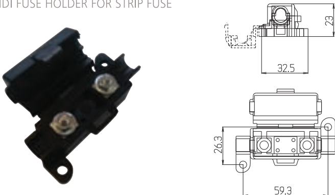
TEKLİ SİGORTA KUTUSU LEVHA TİPİ SİGORTA İÇİN MIDI FUSE HOLDER FOR STRIP FUSE 01-017
