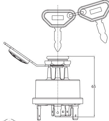
X DETAYI TS 1472 DETAIL X
