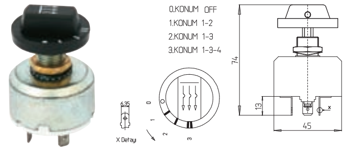
MAGIRUS KALORİFER ANAHTARI (Y.M. ÇEVİRMELİ) 11-018 MAGIRUS HEATING SYSTEM ROTARY SWITCH (NEW MODEL)
