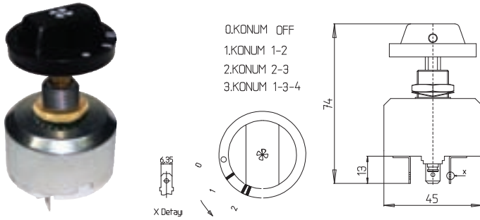
MAGIRUS FAR ANAHTARI (Y.M. ÇEVİRMELİ) 11-017 MAGIRUS HEADLIGHT ROTARY SWITCH (NEW MODEL)
