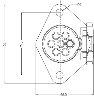
7'Li N TİPİ ALÜMİNYUM TIR RÖMORK FİŞİ (VİDALI) / 7 PIN ALUMINIUM TIR TRAILER SOCKET (N TYPE AND SCREW TERMINAL)
