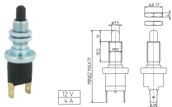
MERCEDES KAMYON FREN OTOMATİĞİ MERCEDES TRUCK STOPLIGHT SWITCH
