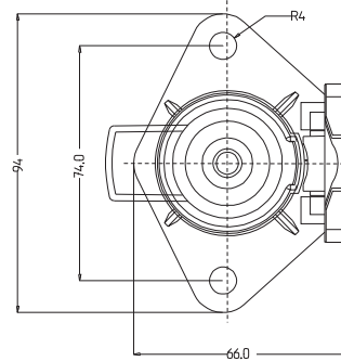
7'Lİ S TİPİ PLASTİK TIR RÖMORK PRİZİ (TERMİNALLİ VE SOKETLİ) / 7 PIN PLASTIC TIR TRAILER SOCKET (S TYPE)
