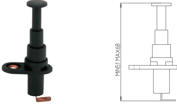
BUTON KAPI VE ALARM İÇİN (PLASTİK UZUN) PUSH BUTTON FOR DOOR AND ALARM (PLASTIC LONG)
