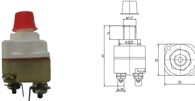
PNÖMATİK FREN OTOMATİĞİ Y.M. (BEDFORD VE KARGO KAMYON) PNEUMATIC BRAKE OIL PRESSURE SWITCH (BEDFORD&CARGO)
