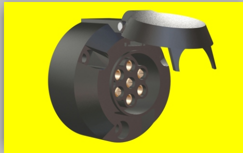
06 0603 PLASTİK RÖMORK FİŞİ DİŞİ 7'LI PLASTIC - TRAILER SOCKET 7'PINS. ISO 1724-DIN 72577-N.
