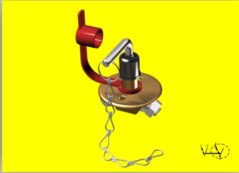
05 0201 METAL DEVRE KESİCİ BATTERY CUT - OFF SWITCH
