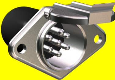
06 0404 ALUMİNYUM RÖMÖRK FİŞİ KOMPLE N TİP ALUMINIUM SOCKET AND PLUG 7 PINS N TYPE ISO 1185-DIN 72579-N. 24V
