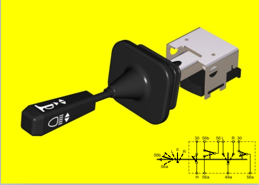
34 0528 MAGIRUS FAR KOLU STEERING COLUMN SWITCH
