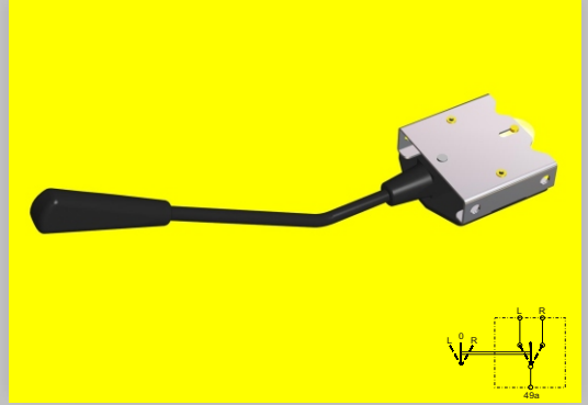
01 1510 RENAULT SİNYAL KOLU SIGNAL SWITCH
