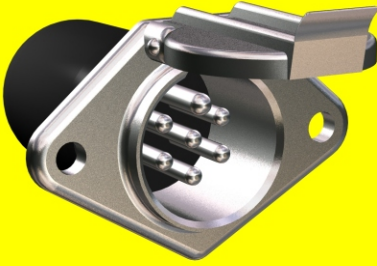
06 0407 ALUMİNYUM RÖMÖRK FİŞİ DİŞİ N TİP ALUMINIUM - TRAILER SOCKET 7 PINS N TYPE ISO 1185-DIN 72579-N. 24V
