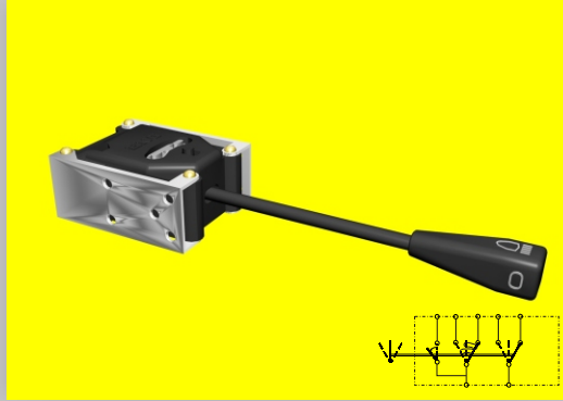
01 1509 RENAULT FAR KOLU 01 1521 TOROS FAR KOLU HEADLIGHT SWITCH
